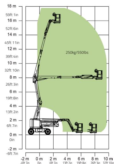
Range of Motion ZA16JERT/ZA16JERT-Li
