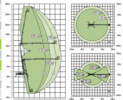
Range of Motion ZX27AE
