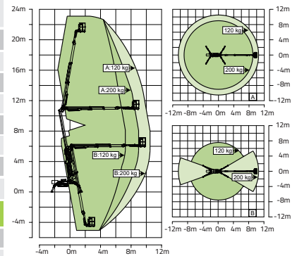
Range of Motion ZX23AE
